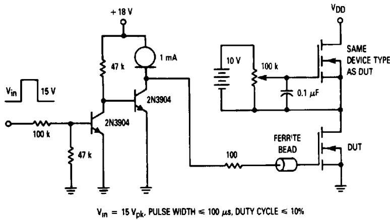
Figure 18. Gate Charge Test Circuit
