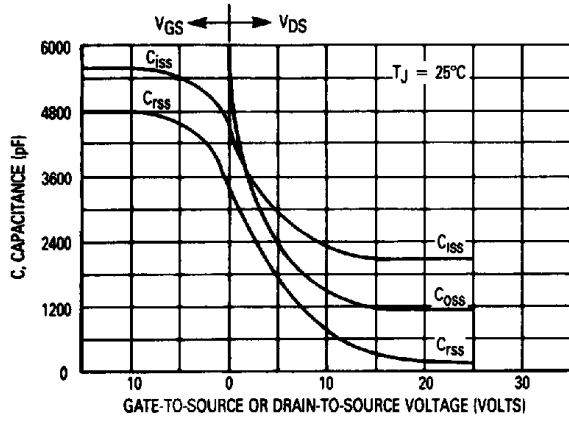
Figure 16. Capacitance Variation
